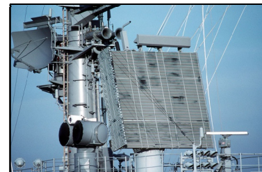
US Navy SPS-48E Radar with Roll-Rings integrated into the high power microwave rotary joint
